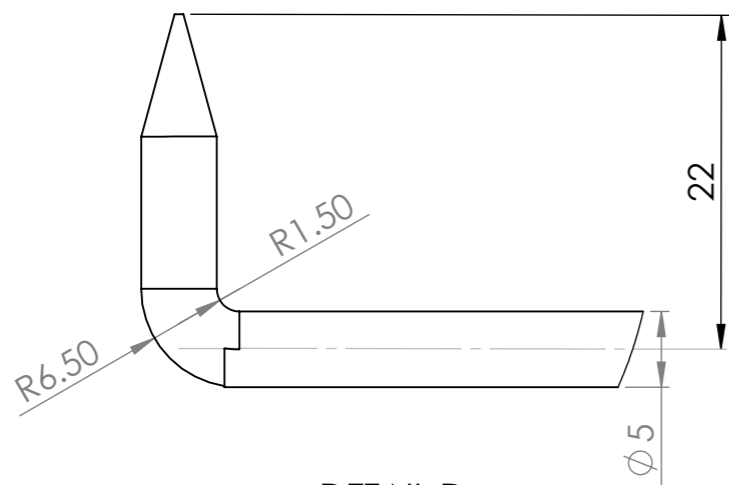
DETAIL D SCALE 2 : 1
