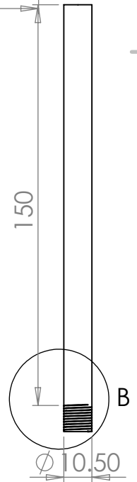
DETAIL B
